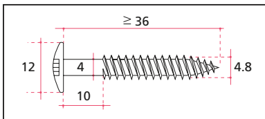
FIG. G — Screw (supplied by AFCC)
