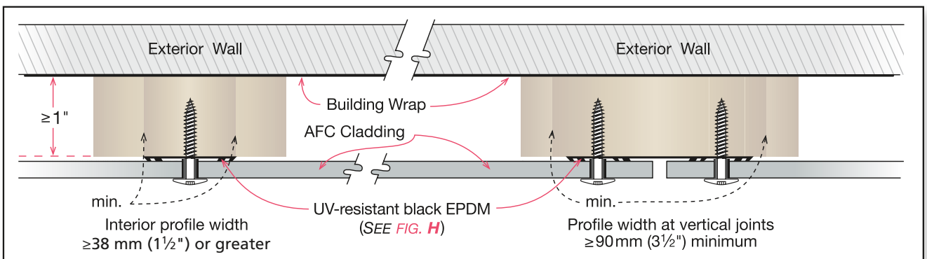
FIG. J — Wood profiles: interior and vertical joint. (Vertical joints may also use two \geq 38\text{mm} profiles in place of one \geq 90\text{mm} profile.)
