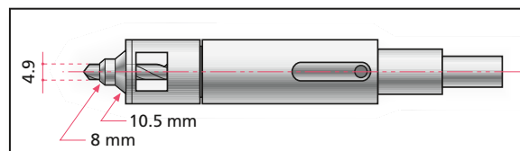
FIG. 1 — Centralizing drill bit
