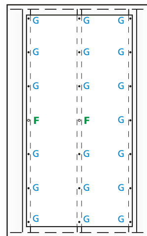
▼ FIG. F — Vertical installation on vertical profiles
