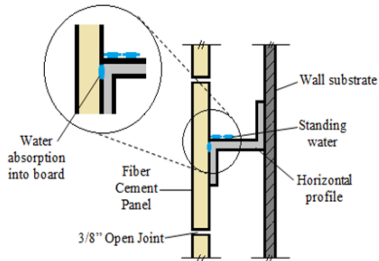
Figure 1: Improper Installation
